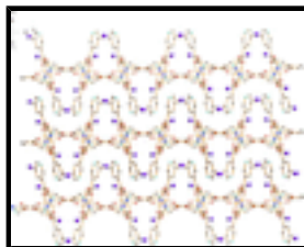
Fig. 3. A view of the packing showing the interdigitation of the pendant 5-bromo-2-pyridyl groups. Color scheme as for Fig. 2.
