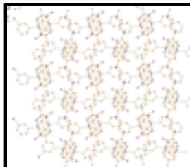
Fig. 1. A view of the two-dimensional structure of [\text{Cu}_2(\text{O}_2\text{CC}_5\text{H}_3\text{NBr})_4] in the bc plane. Color scheme as for Fig. 2.
